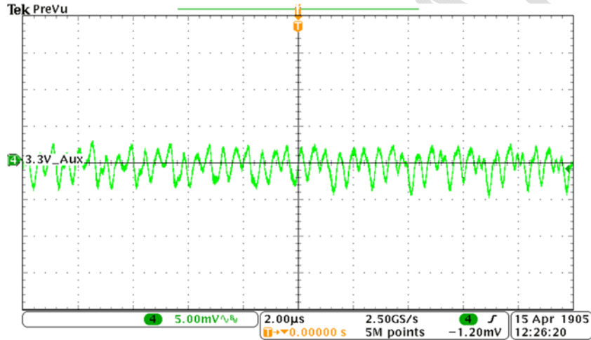
Figure 2: 3.3V Output Ripple
