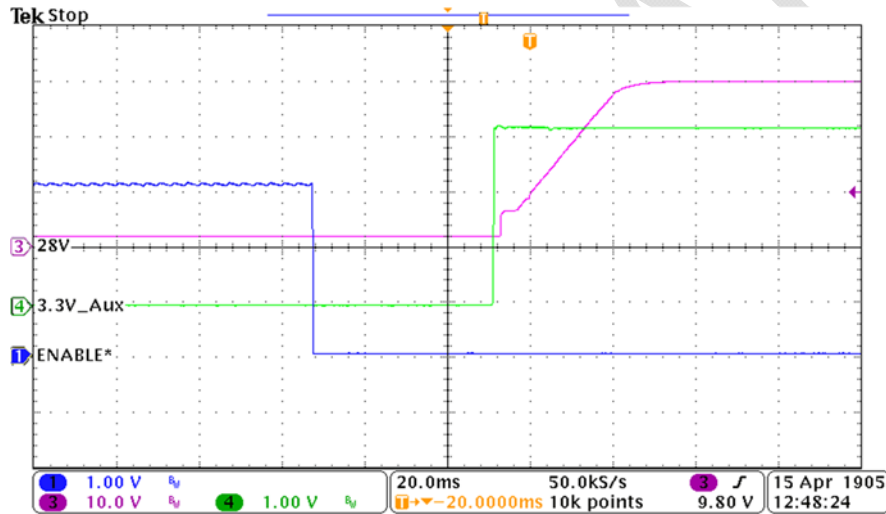
Figure 5: Turn-on sequence 28V, ENABLE* asserted, INHIBIT* de-asserted
