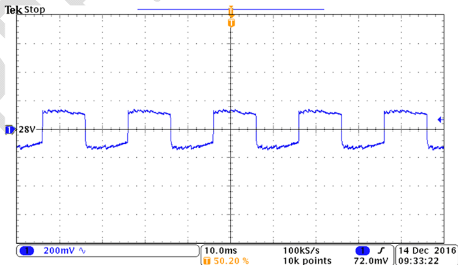
Figure 6: +28V output transient response, 50%-75% load change
