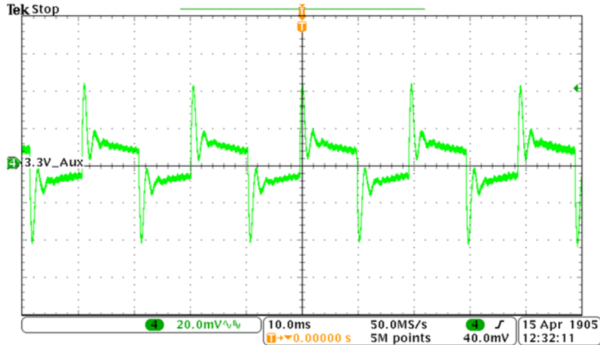
Figure 7: +3.3V output transient response, 50%-75% load change
