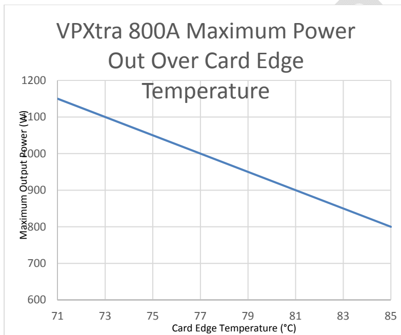
Figure 11: Maximum Output Power over Card Edge Temperature
