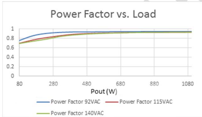
Figure 8: Power Factor vs. Load for Minimum, Nominal and Maximum input voltage
