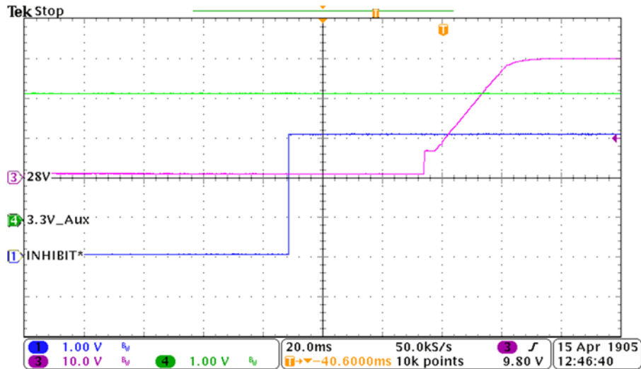
Figure 1: Turn-on delay from INHIBIT* de-assertion, main outputs
