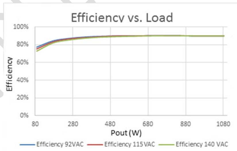
Figure 9: Efficiency vs. Load for Minimum, Nominal and Maximum input voltage
