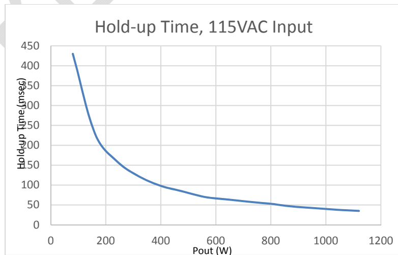
Figure 11: Hold-up Time at 115VAC Input with VPXtra HU700HV
