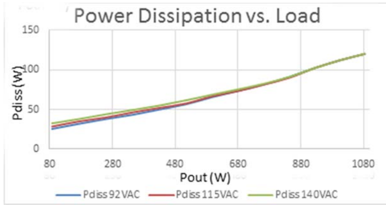
Figure 10: Power dissipation vs. Load for Minimum, Nominal and Maximum input voltage
